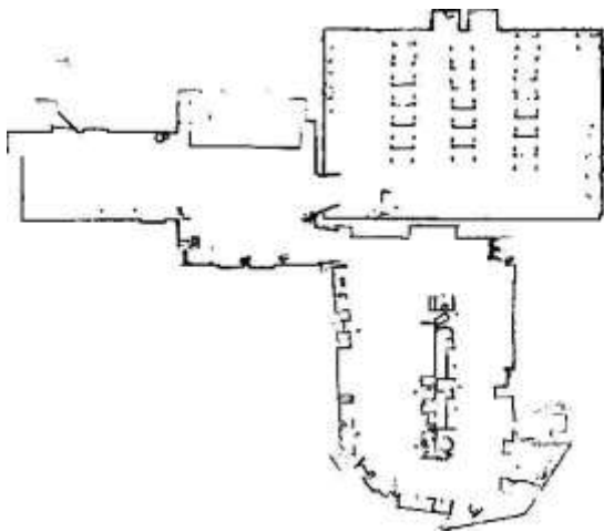
Figure 6(a): Map obtained using LIDAR
