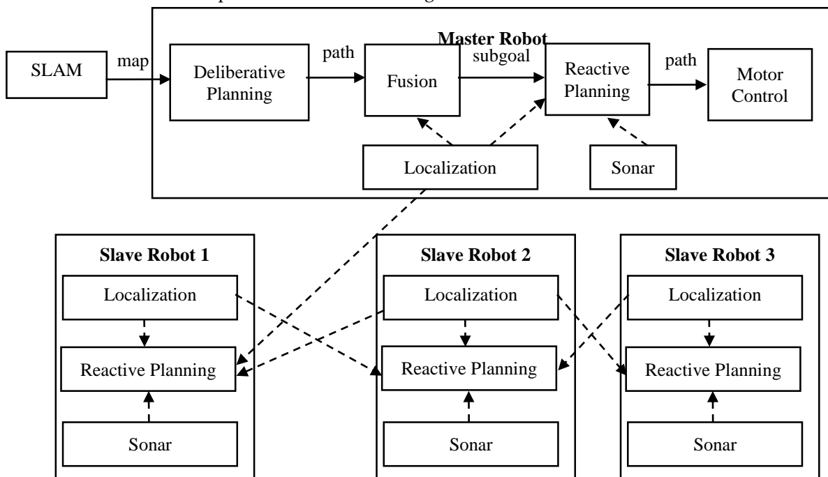
Figure 4: Overall Solution Architecture.
