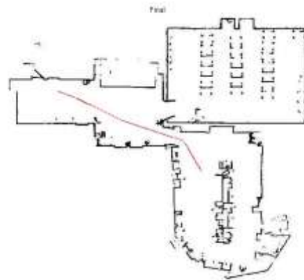
Figure 7(b): The final path found after applying the A* algorithm.
