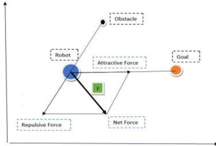
Figure 3: The forces on the robot.
